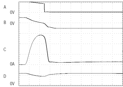
SLOW CURRENT-LIMIT RESPONSE
