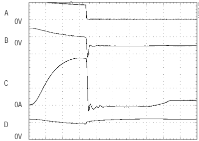
FAST CURRENT-LIMIT RESPONSE
