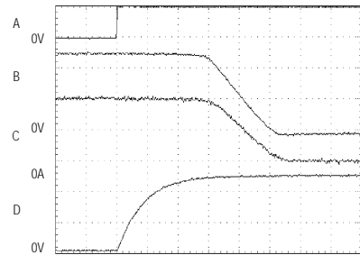
SWITCH TURN-OFF TIME
