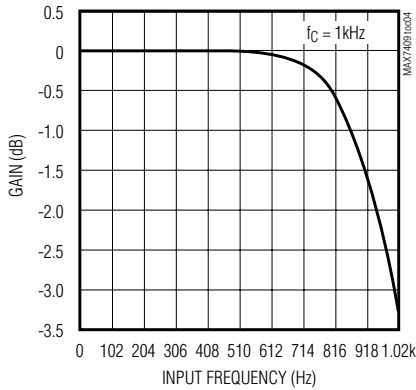
MAX7410/MAX7414 PASSBAND FREQUENCY RESPONSE (BUTTERWORTH)
