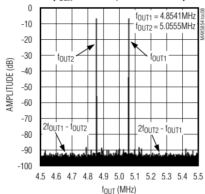
TWO-TONE INTERMODULATION DISTORTION ( f_{CLK} = 165MHz , 1MHz WINDOW)
