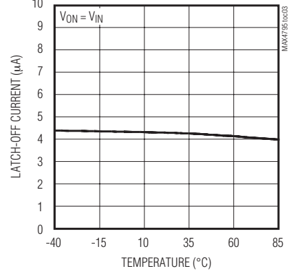
LATCH-OFF LEAKAGE CURRENT vs. TEMPERATURE
