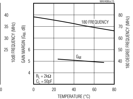
GAIN MARGIN AND 180 DEGREE FREQUENCY vs. TEMP (Av = 10dB)
