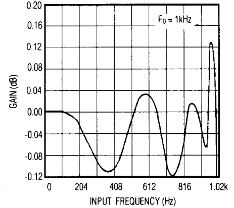
MAX297 PASSBAND FREQUENCY RESPONSE
