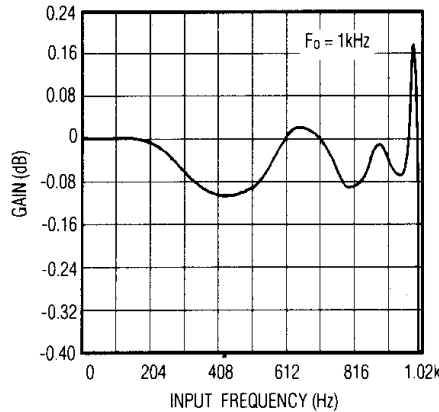
MAX294 PASSBAND FREQUENCY RESPONSE
