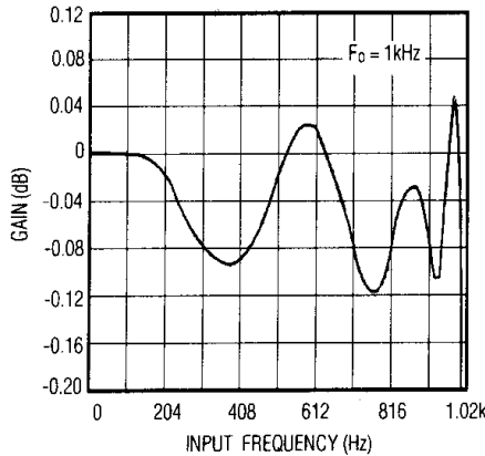
MAX293 PASSBAND FREQUENCY RESPONSE
