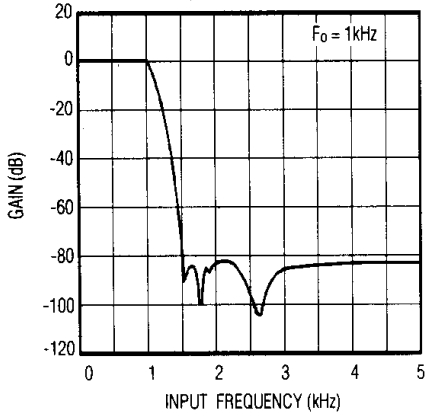
MAX293 PASSBAND FREQUENCY RESPONSE
