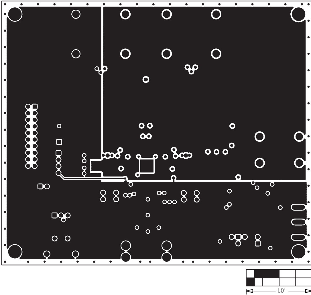
Figure 6. MAX9744 EV Kit PCB Layout—Layer 3 (Power)
