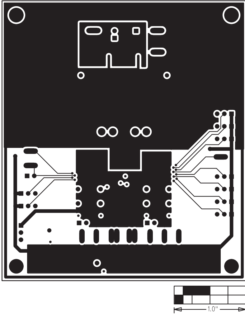
Figure 6. MAX9709 EV Kit PCB Layout—VDD Layer 3
