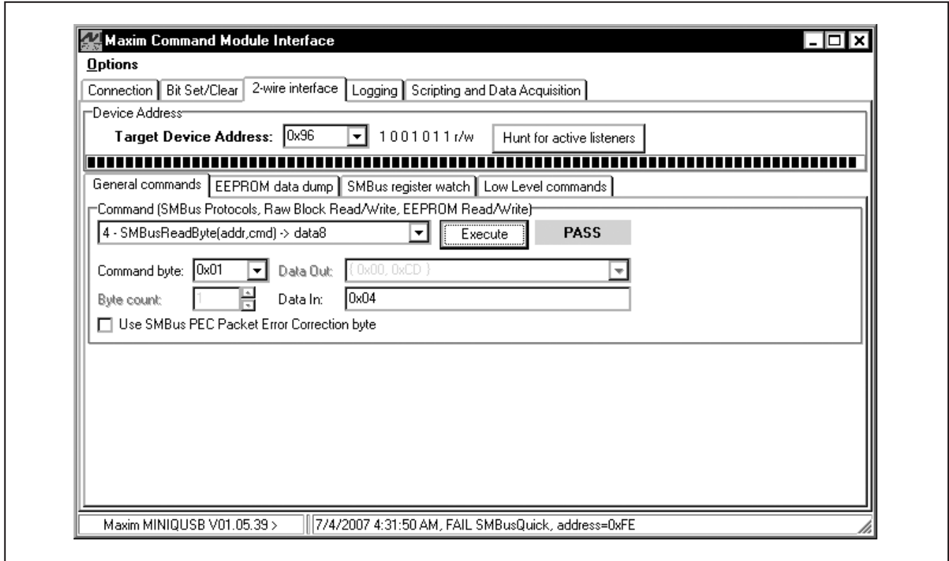
Figure 4. Example of a Simple SMBusReadByte Operation Using the Advance User Interface
