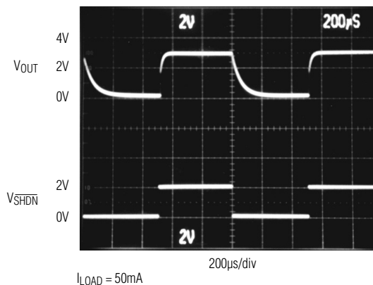
MAX8864 SHUTDOWN
