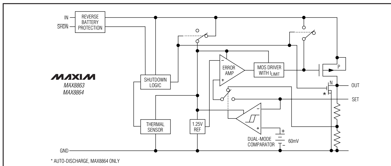
Figure 1. Functional Diagram
