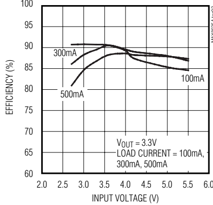
SKIP-MODE EFFICIENCY vs. INPUT VOLTAGE
