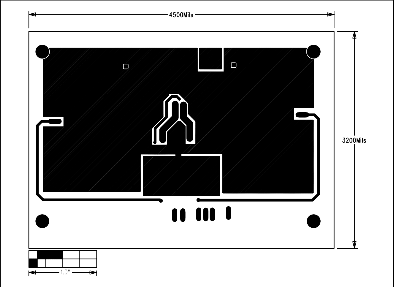
Figure 4. MAX8529 EV Kit PC Board Layout—Solder Side
