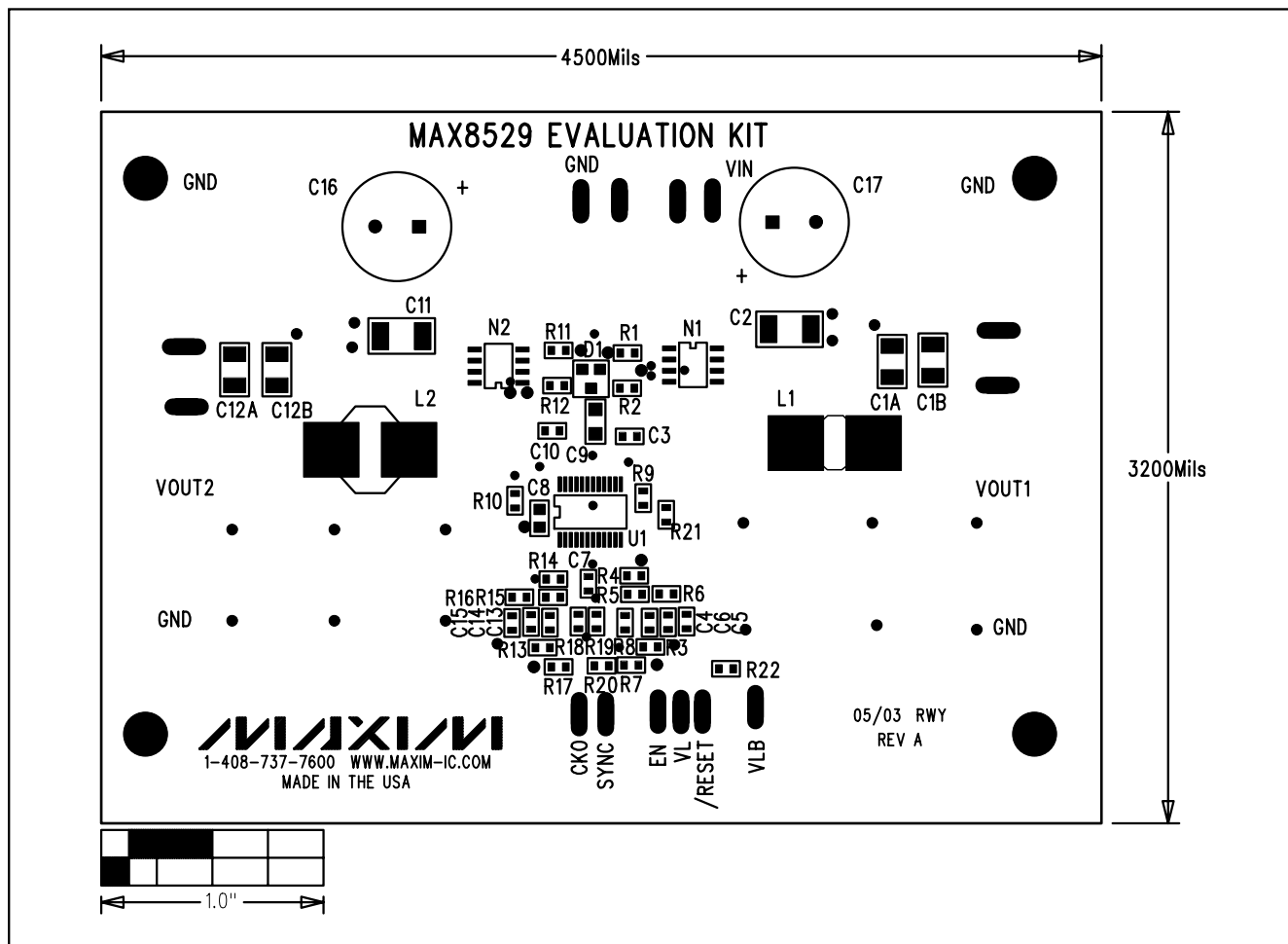
Figure 2. MAX8529 EV Kit Component Placement Guide—Top Silkscreen
