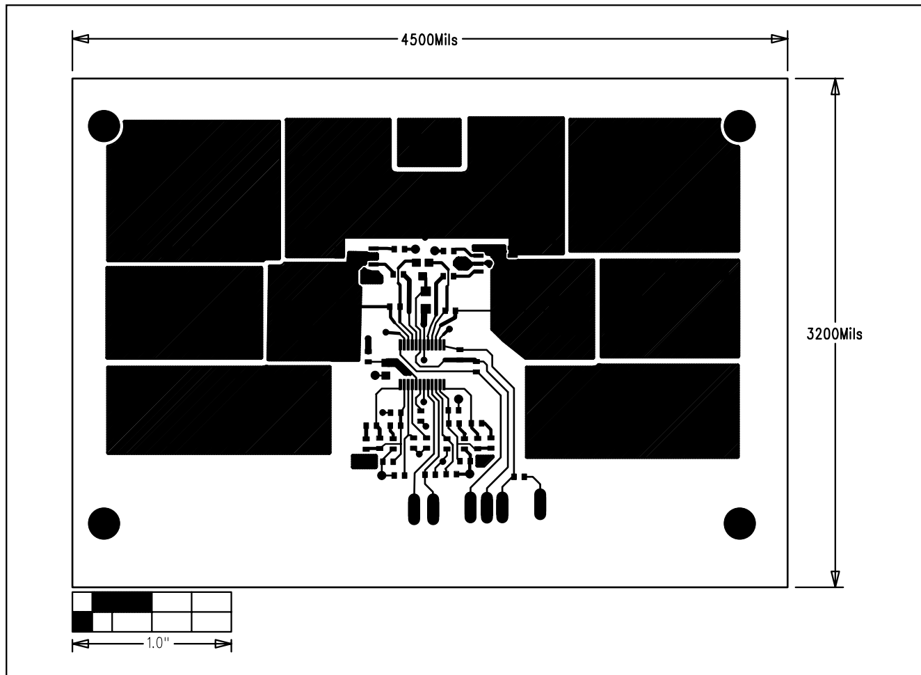
Figure 3. MAX8529 EV Kit PC Board Layout—Component Side
