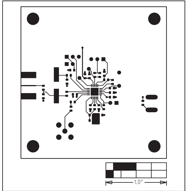
Figure 4. MAX7036 EV Kit PCB Layout—Component Side
