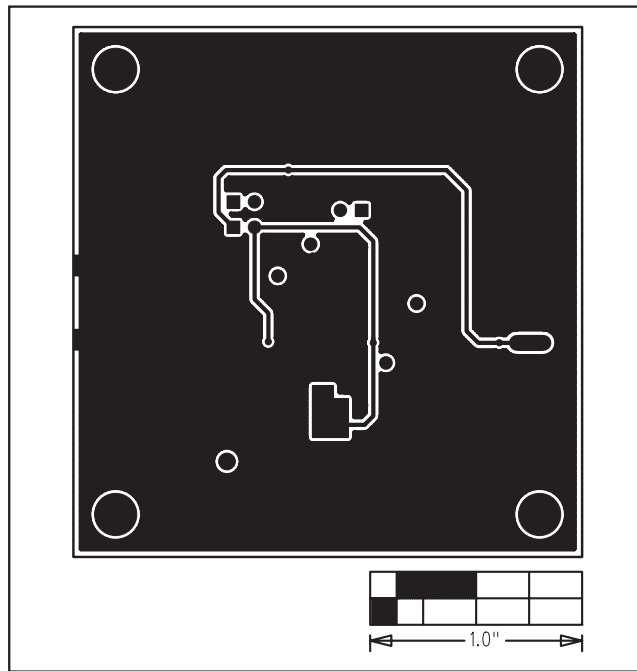
Figure 5. MAX7036 EV Kit PCB Layout—Solder Side
