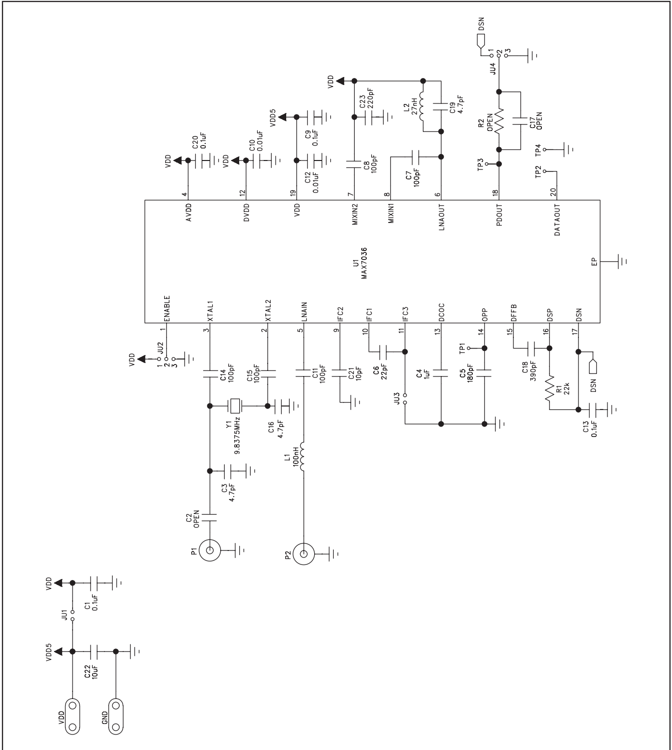
Figure 1. MAX7036EVKIT315+ EV Kit Schematic
