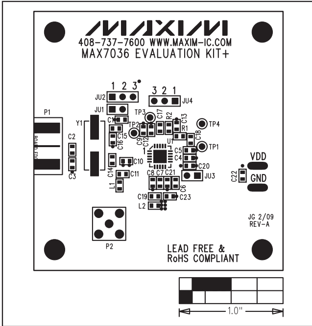
Figure 3. MAX7036 EV Kit Component Placement Guide—Component Side
