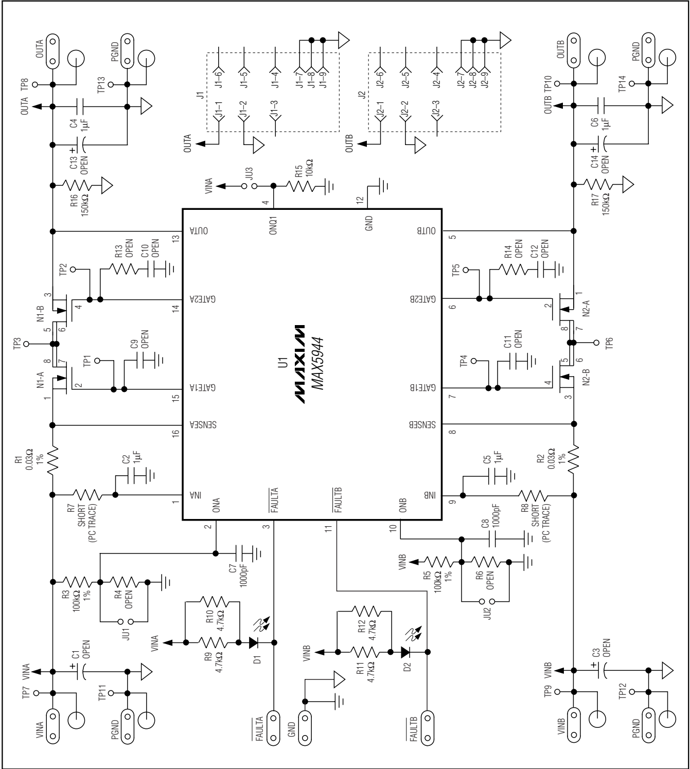
Figure 1. MAX5944 EV Kit Schematic
