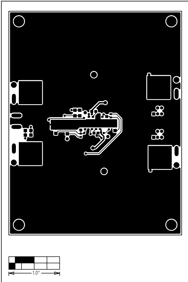
Figure 4. MAX5944 EV Kit PC Board Layout—Solder Side
