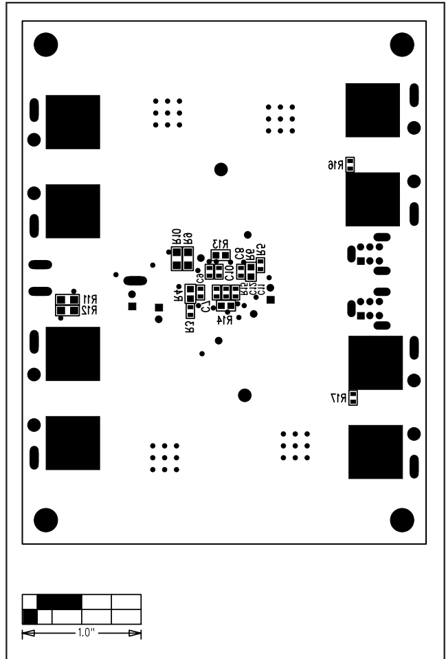
Figure 5. MAX5944 EV Kit Component Placement Guide—Solder Side
