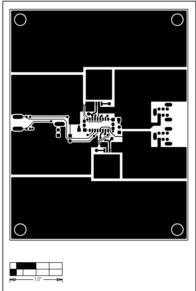
Figure 3. MAX5944 EV Kit PC Board Layout—Component Side
