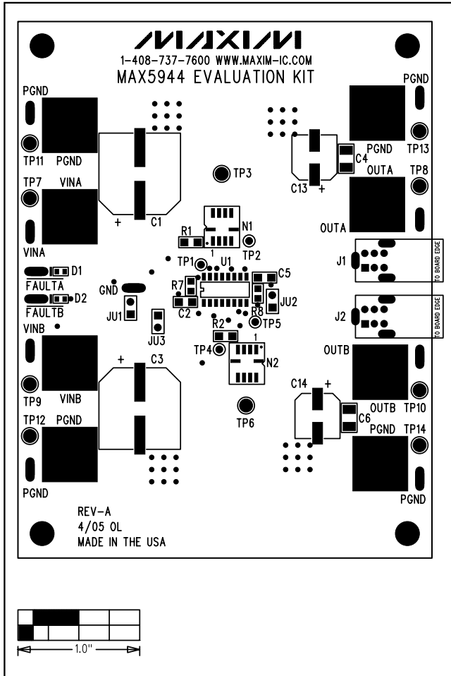
Figure 2. MAX5944 EV Kit Component Placement Guide—Component Side
