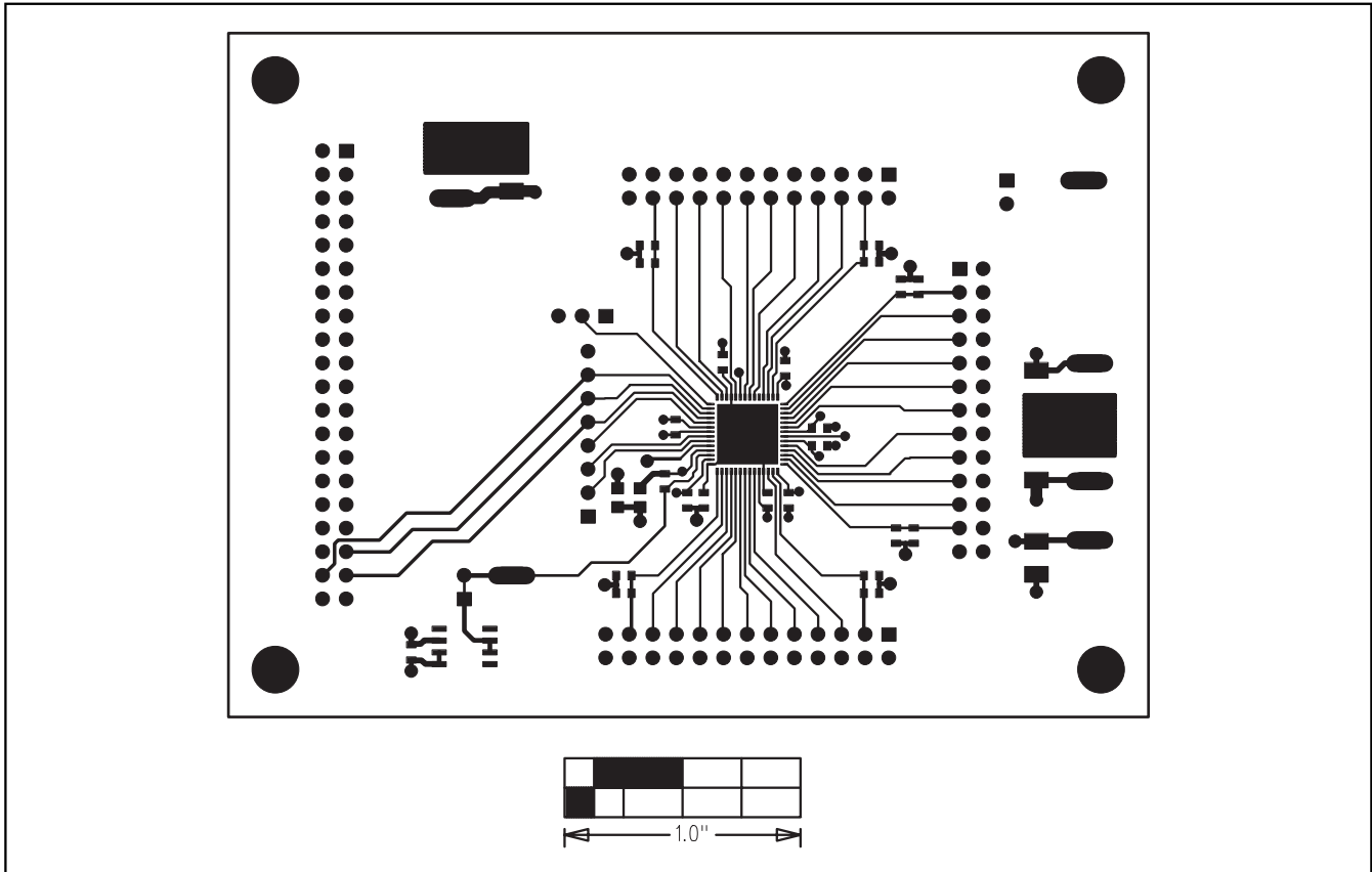
Figure 7. MAX5734 EV Kit PCB Layout—Component Side
