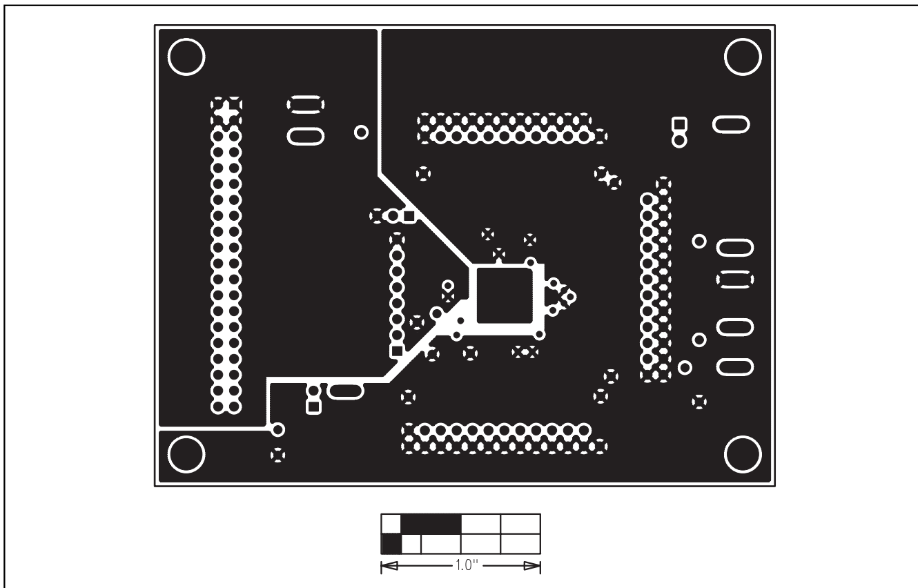
Figure 8. MAX5734 EV Kit PCB Layout—Ground Layer
