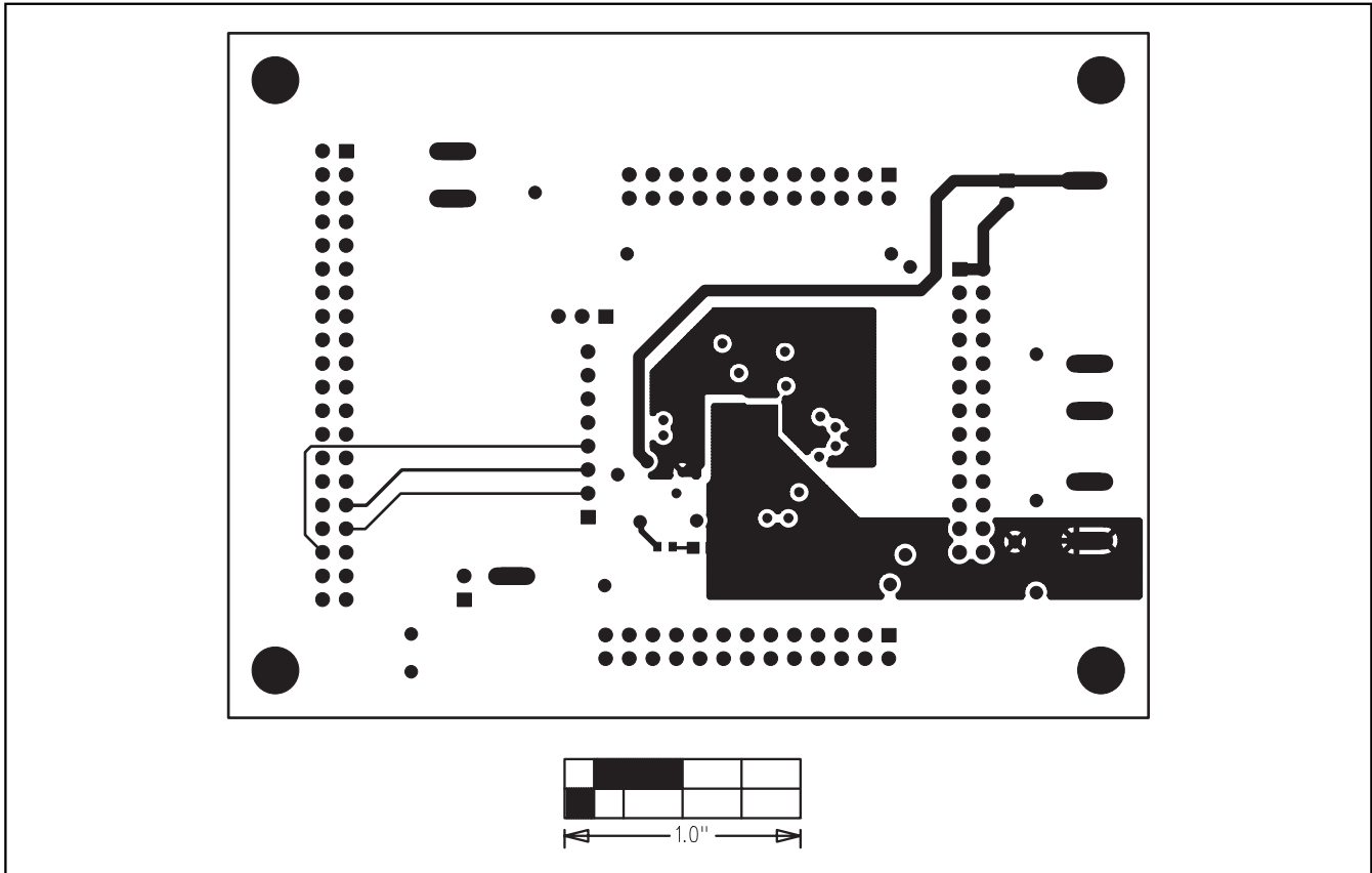
Figure 10. MAX5734 EV Kit PCB Layout—Solder Side
