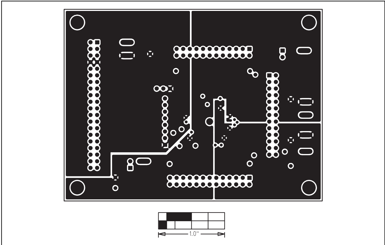
Figure 9. MAX5734 EV Kit PCB Layout—Power Layer
