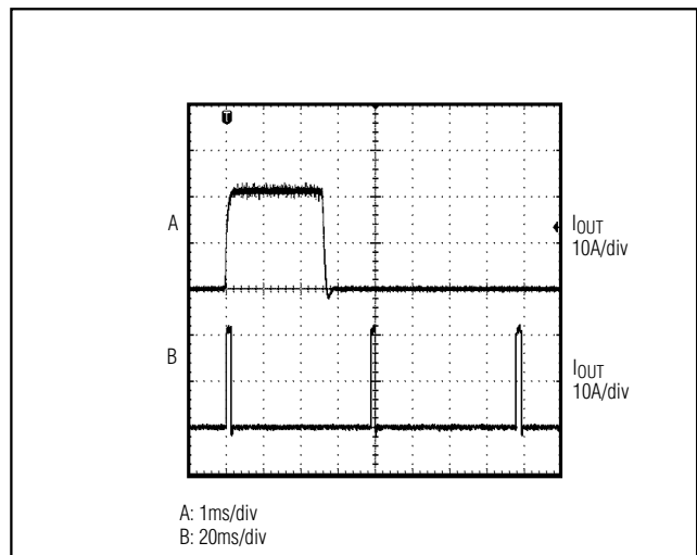
Figure 8. Load Current (10A/div) as a Function of Time when Converter Attempts to Turn On into a 0.050\Omega Short Circuit (Also Acts as Current-Sense Resistor)
