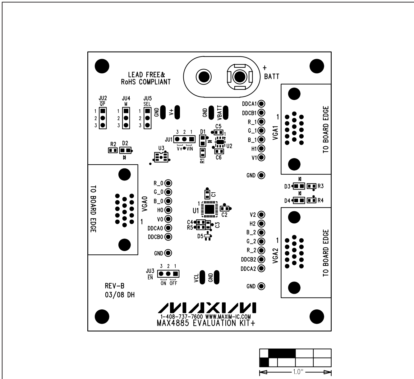
Figure 2. MAX4885 EV Kit Component Placement Guide—Top Silkscreen
