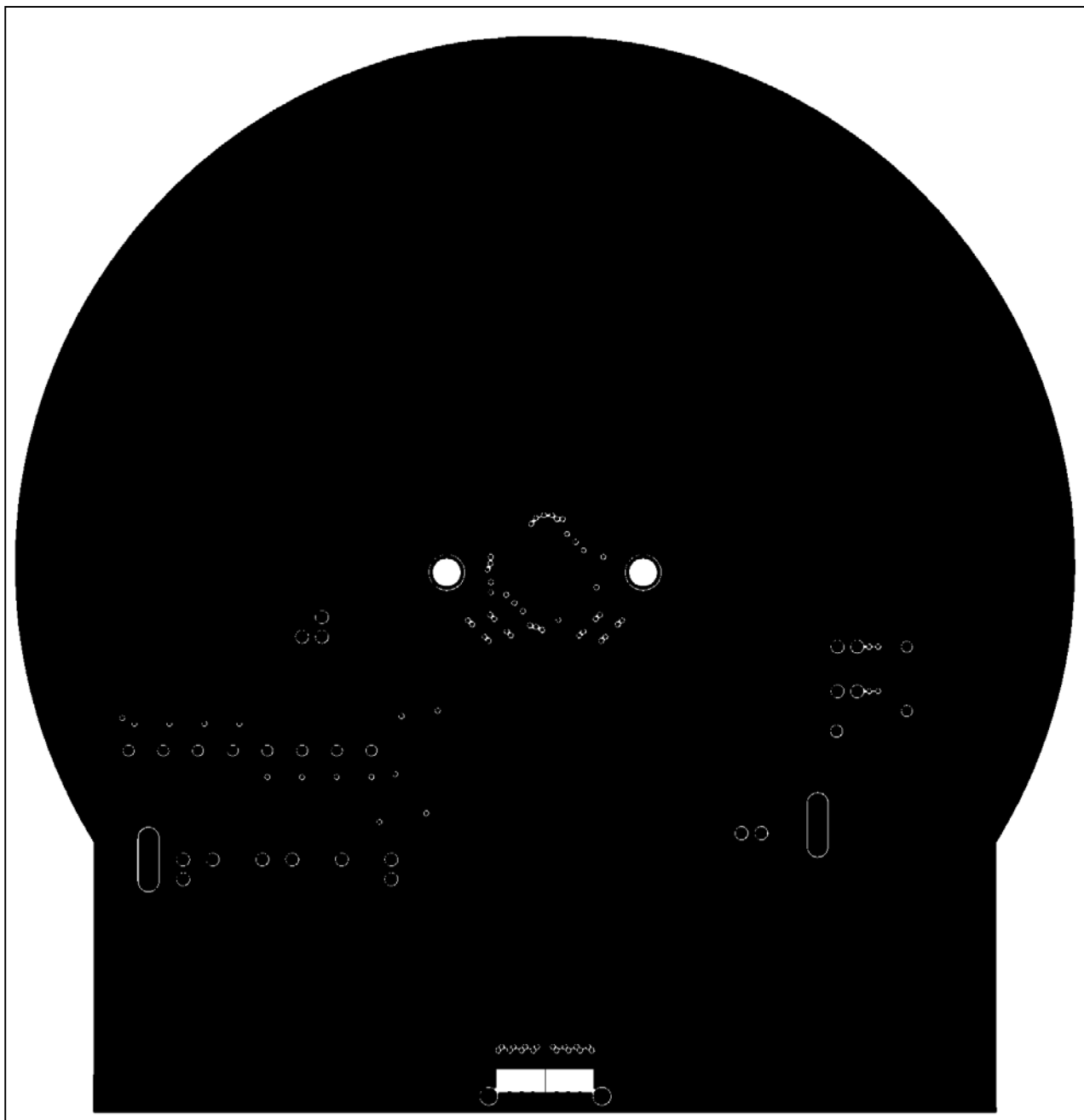
Figure 4. MAX3983 EV Kit PC Board Layout – Ground Plane, Layer 2
