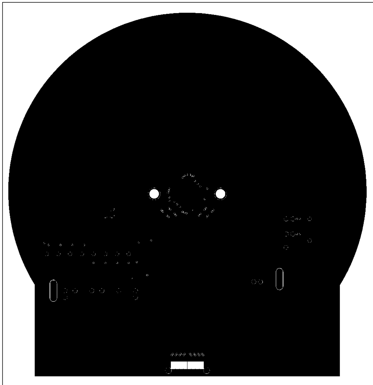
Figure 6. MAX3983 EV Kit PC Board Layout – Ground Plane, Layer 4
