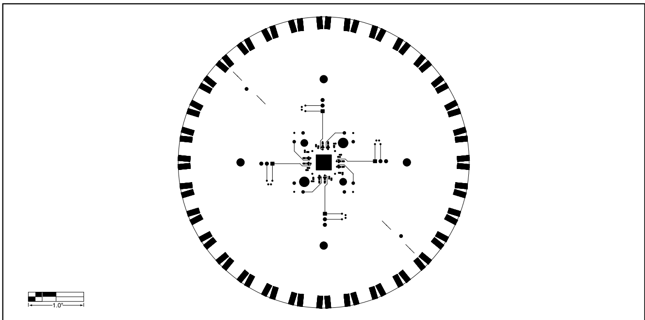
Figure 7. MAX3802 EV Kit PC Board Layout—Solder Side
