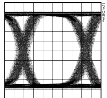
EQUALIZER OUTPUT EYE DIAGRAM AFTER 72ft OF 75Ω RG179 CABLE (300mVp-p SINGLE ENDED, 2^{23} - 1 PRBS)
