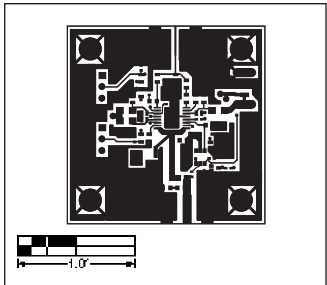
Figure 10. MAX2269 EV Kit PC Board Layout—Component Side
