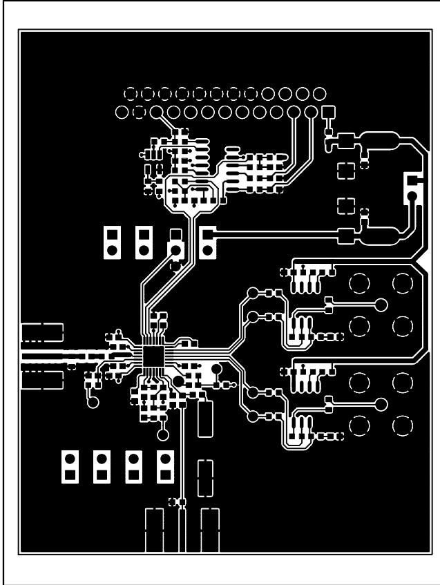
Figure 3. MAX2112 EV Kit PCB Layout—Top
