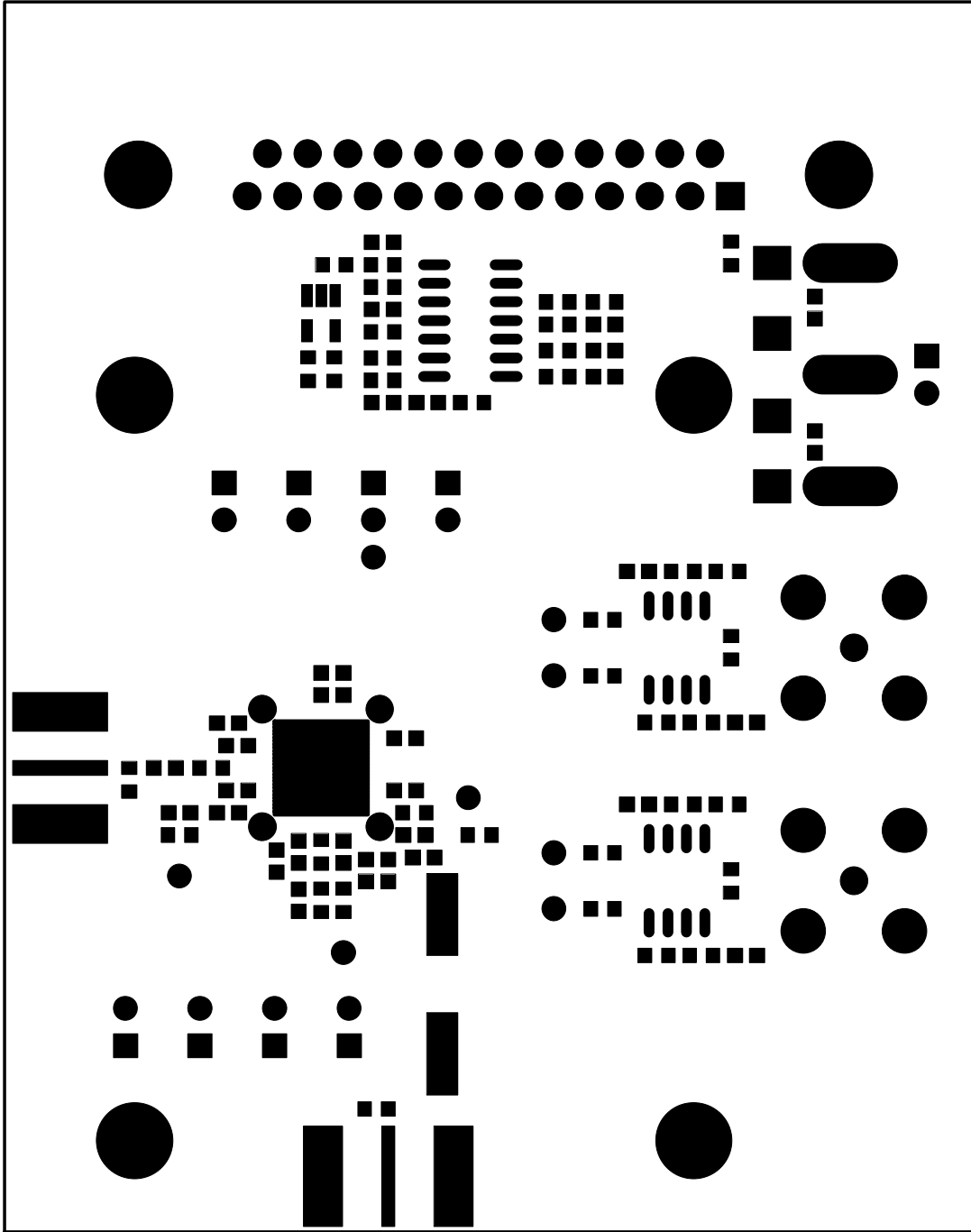
Figure 5. MAX2112 EV Kit PCB Layout—Top Soldermask
