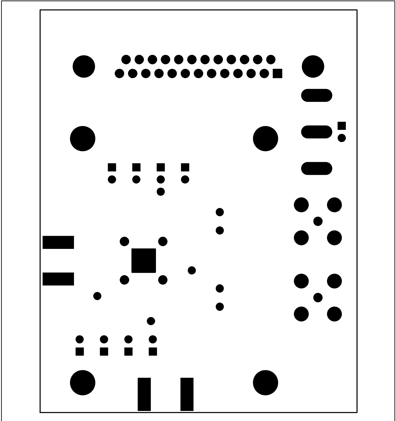
Figure 6. MAX2112 EV Kit PCB Layout—Bottom Soldermask
