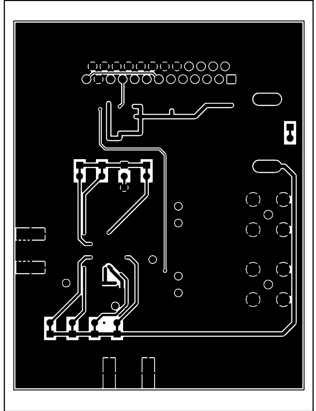
Figure 4. MAX2112 EV Kit PCB Layout—Bottom
