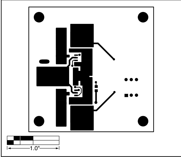
Figure 7. MAX1761 EV Kit PC Board Layout—Component Side
