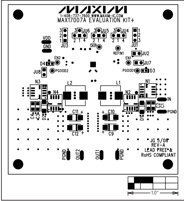
Figure 2. MAX17007A EV Kit Component Placement Guide—Component Side
