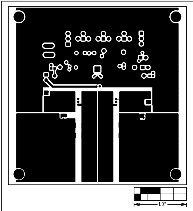
Figure 3. MAX17007A EV Kit PCB Layout—Component Side
