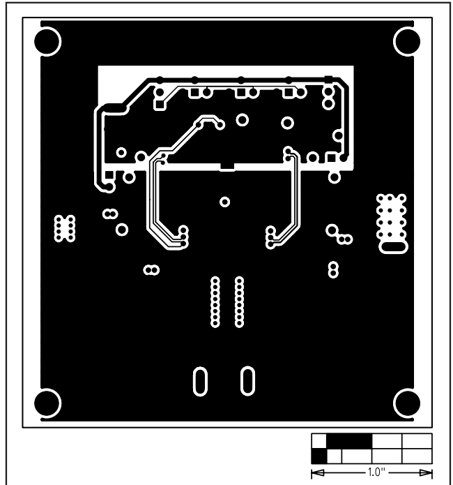
Figure 5. MAX17007A EV Kit PCB Layout—GND Layer 3
