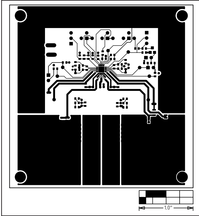
Figure 6. MAX17007A EV Kit PCB Layout—Solder Side
