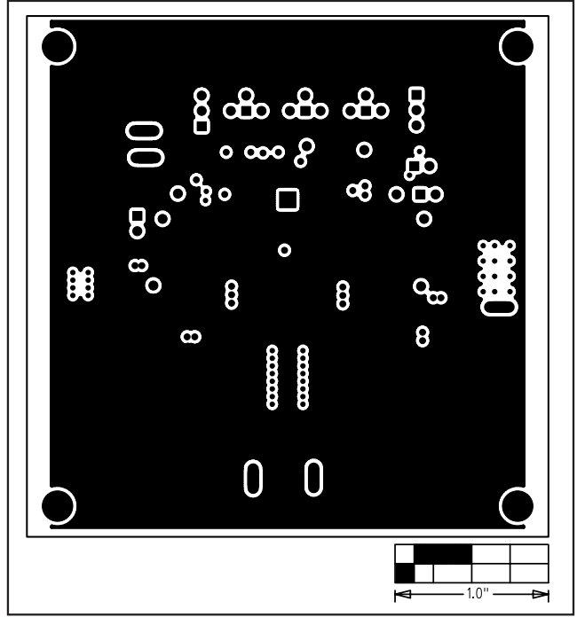
Figure 4. MAX17007A EV Kit PCB Layout—GND Layer 2
