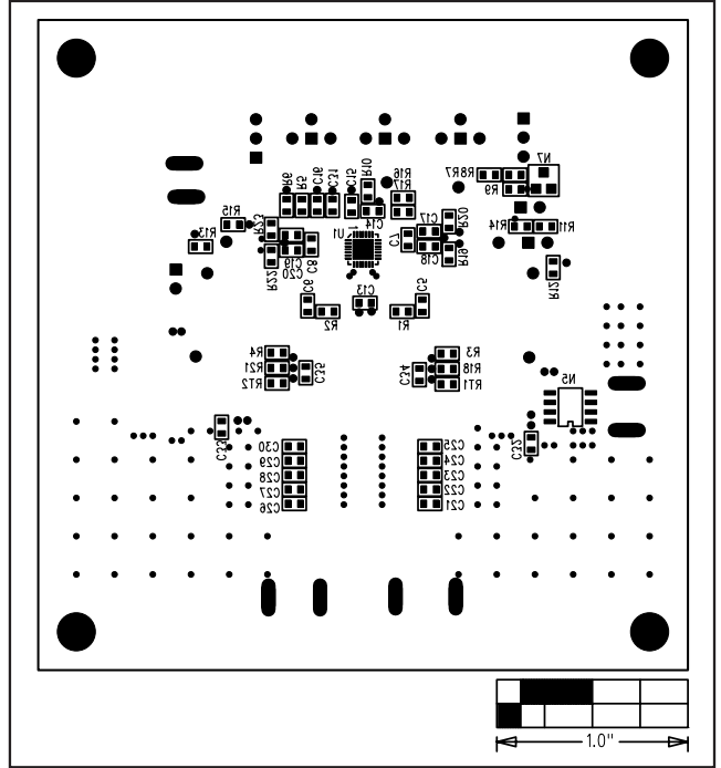
Figure 7. MAX17007A EV Kit Component Placement Guide—Solder Side
