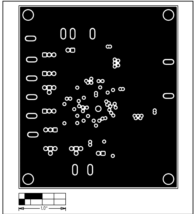
Figure 5. MAX1541 EV Kit PC Board Layout—Ground Layer 2
