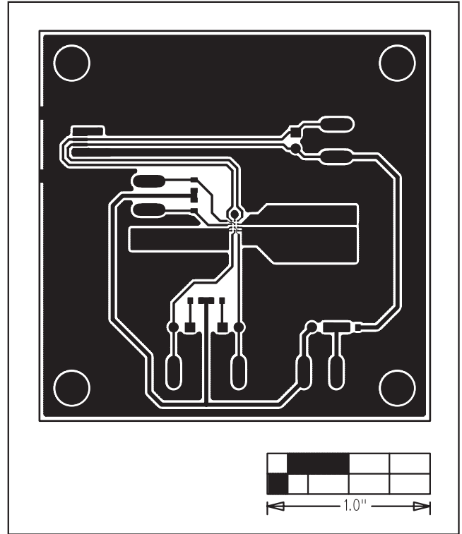
Figure 3. MAX14529E EV Kit PCB Layout—Component Side
