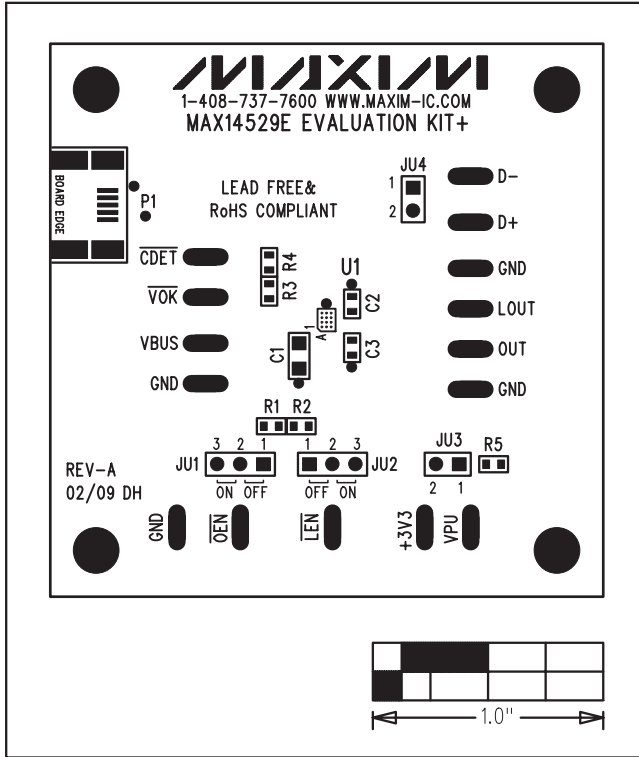
Figure 2. MAX14529E EV Kit Component Placement Guide—Component Side
