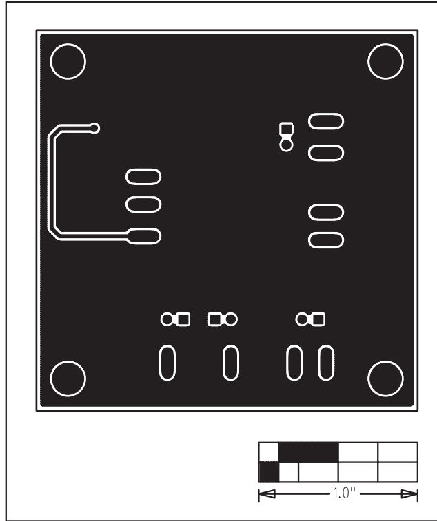
Figure 4. MAX14529E EV Kit PCB Layout—Solder Side
