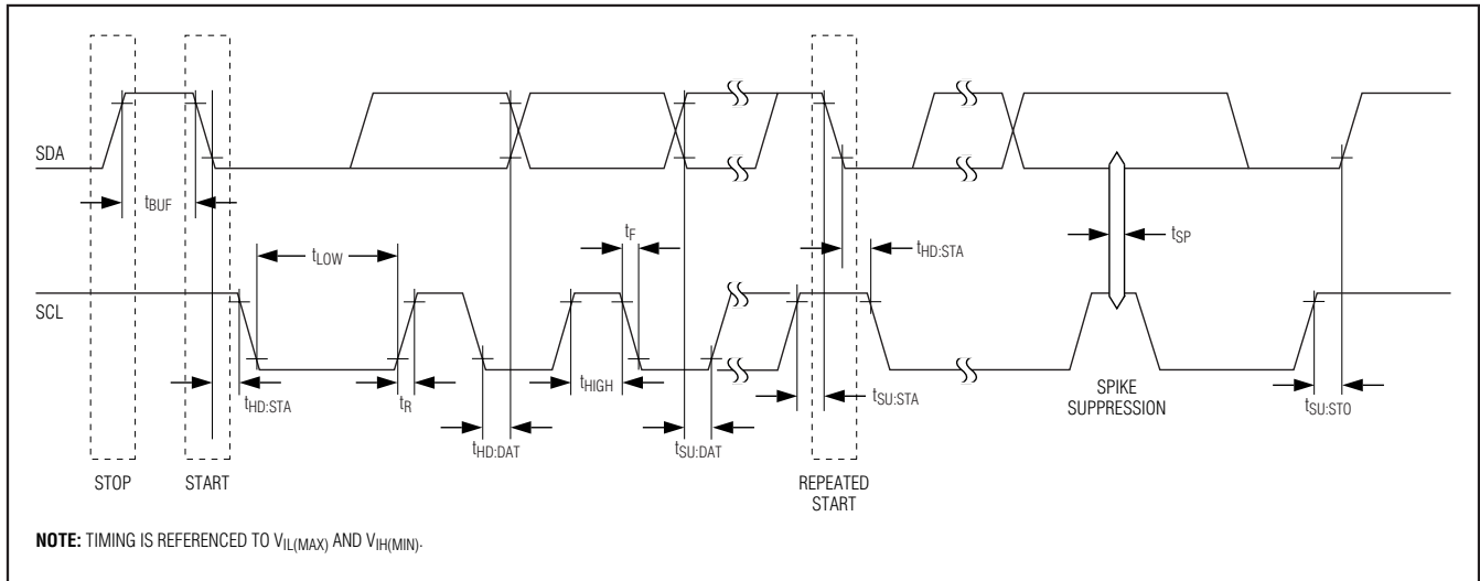
Figure 10. I 2 C Timing Diagram
