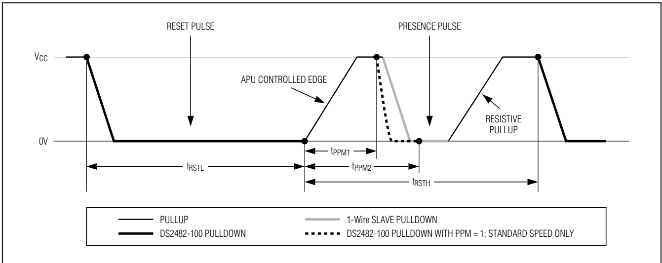
Figure 3. Presence-Pulse Masking
