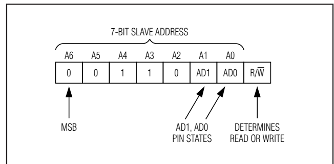
Figure 9. DS2482-100 Slave Address
