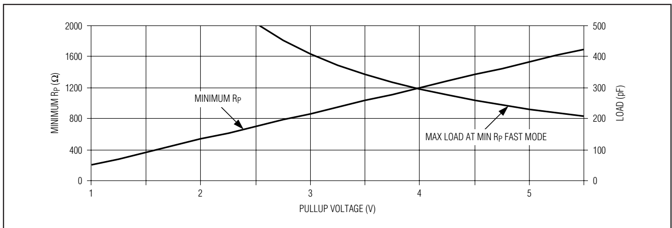
Figure 12. I 2 C Fast Speed Pullup Resistor Selection Chart
