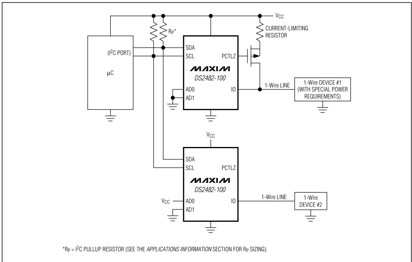
Figure 11. Application Schematic
