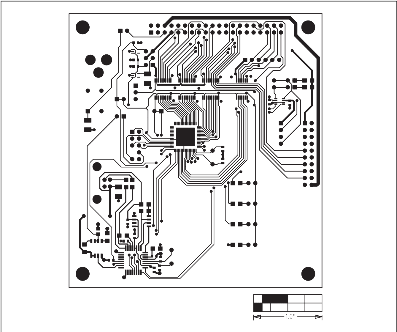
Figure 4. CMAXQUSB PC Board Layout—Component Side
