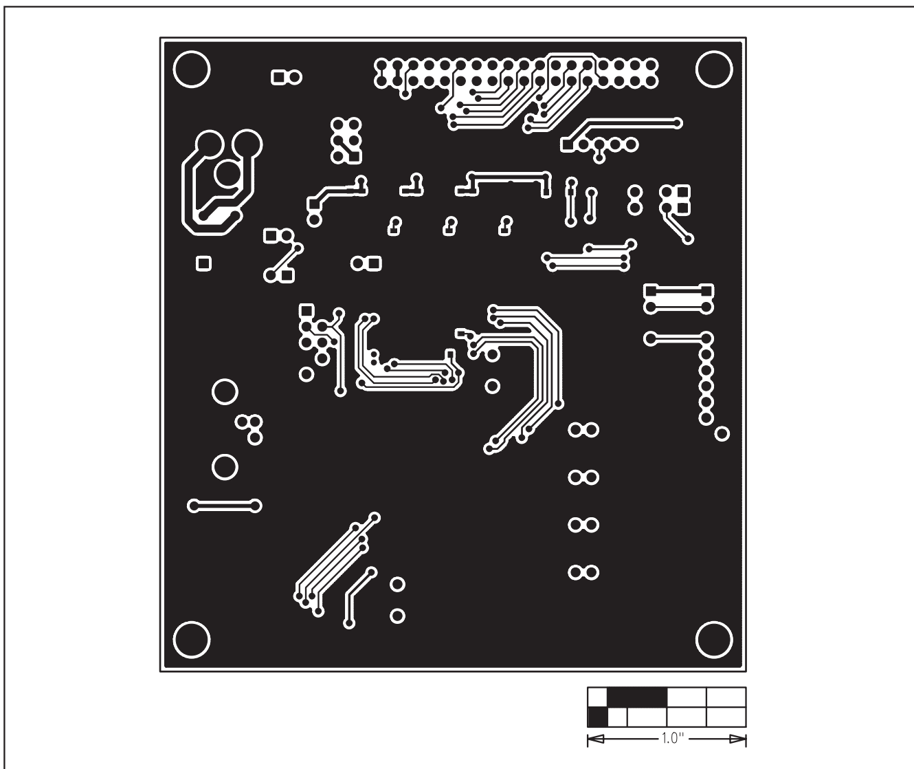
Figure 5. CMAXQUSB PC Board Layout—Solder Side
