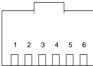
Looking into Female RJ11 Connector
